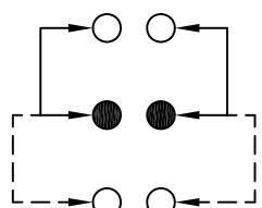
SCHEMATIC (NON-SHORTING)
